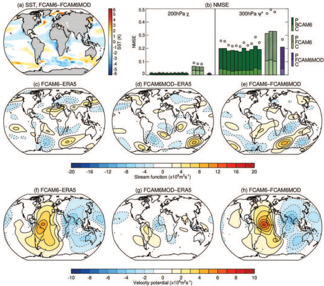
Figure 11. (a) The difference between the JJA climatology of the observed SSTs prescribed in FCAM6 and that of the modeled SSTs from the BCAM6 member used to provide SSTs for FCAM6MOD. (b) the JJA NMSE and SVR for (left) global 200-hPa velocity potential and (right) 300-hPa NH eddy stream function for BCAM6 and FCAM6 (repeated from Figures 8h and 10h) and for FCAM6MOD (purple). (c–e) The 300-hPa eddy stream function for FCAM6-ERA5, FCAM6MOD-ERA5, and FCAM6-FCAM6MOD, respectively. (f–h) As in (c)–(e) but for 200-hPa velocity potential.
