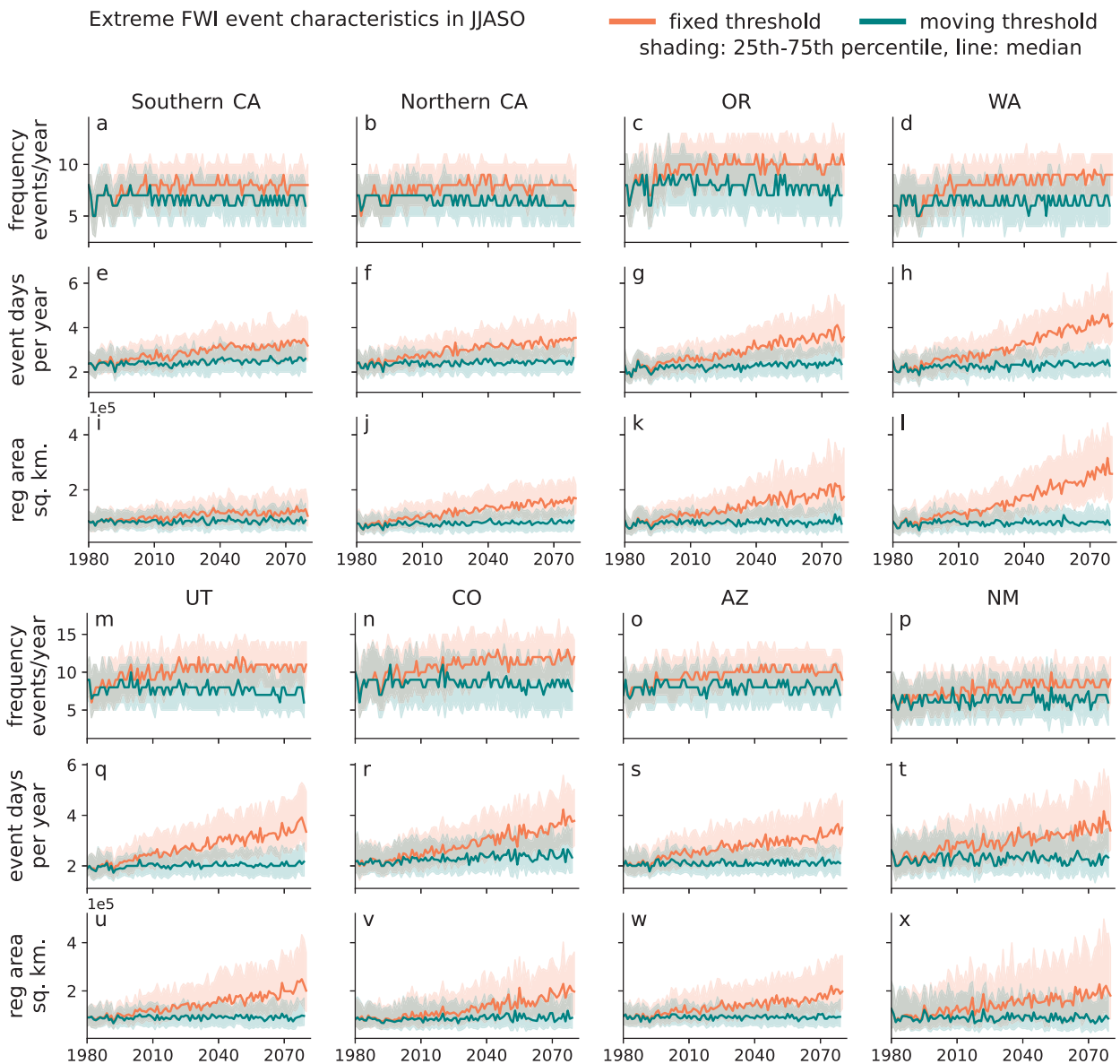
FIG. 4. (a)–(d), (m)–(p) Frequency, (e)–(h), (q)–(t) duration, and (i)–(l), (u)–(x) state-bound area of extreme fire weather events using a fixed (coral) and moving (teal) 99th percentile threshold for events in the (a)–(l) Pacific Coast and (m)–(x) Four Corners regions for JJASO.
