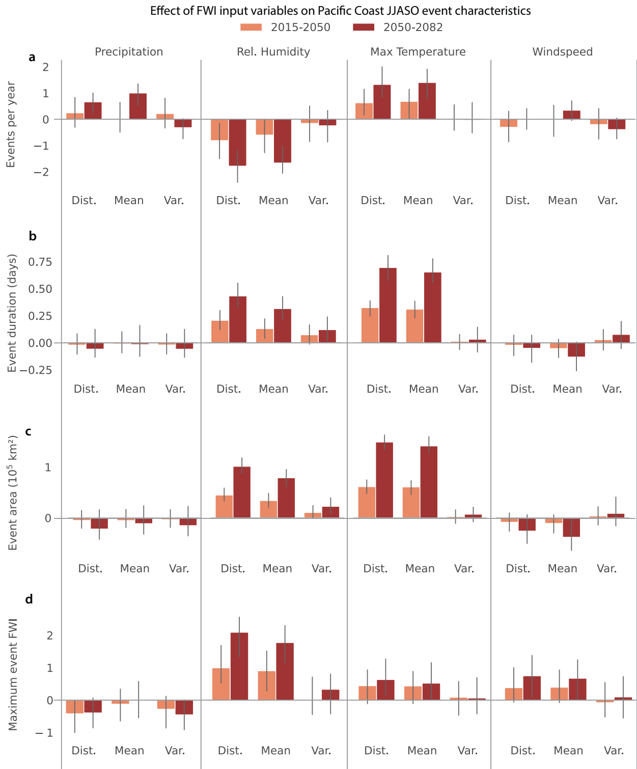
FIG. 10. The difference (from the historic period, 1980–2014) in the impact of changes in the full distribution (Dist.), mean, and variability (Var.) of precipitation, relative humidity, maximum temperature, and wind speed on (a) events per year, (b) events days per year, (c) regional event area, and (d) maximum regional event intensity FWI using the fixed threshold for the early (2015–50, coral) and late future periods (2050–82, red) for the Pacific Coast region in JJASO (see supplemental Fig. 2 for details of the effect calculation for each FWI variable). The mean across all events for each ensemble member is first calculated, and we show the median across all ensemble members. The error bar represents 25th–75th percentile of the ensemble spread.
