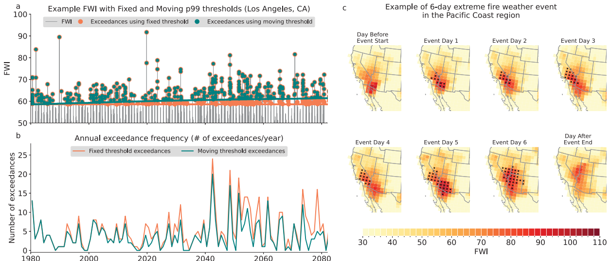
FIG. 1. (a) Example FWI time series for one grid point near Los Angeles and one ensemble member (1001.001), with fixed and moving 99th percentile thresholds and identified exceedances. (b) Annual number of exceedances calculated from (a) fixed and moving thresholds. (c) Example of a 6-day extreme fire weather event over the Pacific Coast region. The shading represents the value of FWI, and the black dots represent the identified spatiotemporally connected event. The event starts when at least one grid point in the regional boundary of the Pacific Coast region (shown in Fig. 3) exceeds the local threshold, and the event ends when there are no longer any grid points that are spatiotemporally connected to that event within the region boundary.
