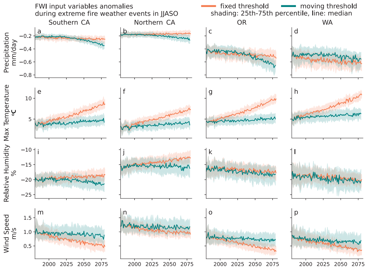
FIG. 6. Time series of (a)–(d) precipitation, (e)–(h) maximum temperature, (i)–(l) relative humidity, and (m)–(p) wind speed anomalies during extreme fire weather events in JJASO in (a),(e),(i),(m) Southern CA, (b),(f),(j),(n) Northern CA, (c),(g),(k),(o) OR, and (d),(h),(l),(p) WA using the fixed mean and threshold (coral) and the moving mean and threshold (teal).
