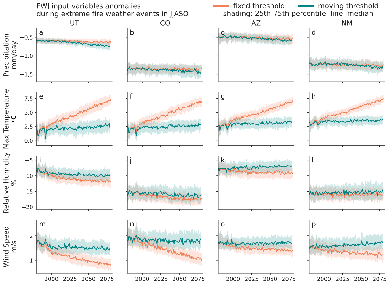
FIG. 8. Time series of (a)–(d) precipitation, (e)–(h) maximum temperature, (i)–(l) relative humidity, and (m)–(p) wind speed anomalies during extreme fire weather events in JJASO in (a),(e),(i),(m) UT, (b),(f),(j),(n) CO, (c),(g),(k),(o) AZ, and (d),(h),(l),(p) NM using the fixed mean and threshold (coral) and the moving mean and threshold (teal).
