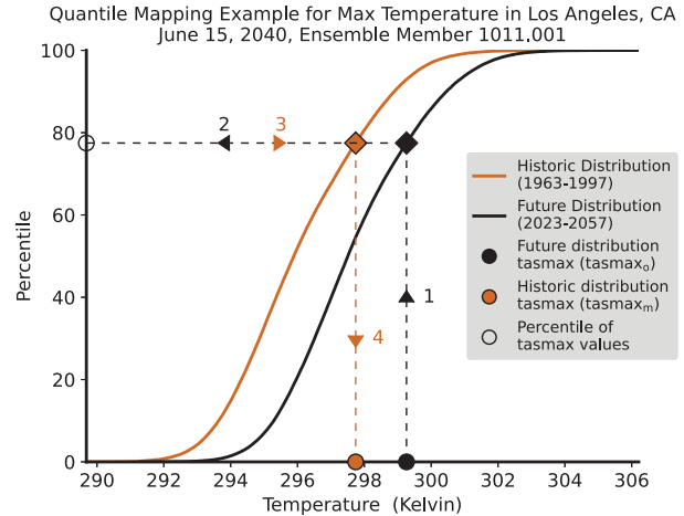
FIG. 2. Schematic of quantile mapping for maximum temperature for 15 Jun 2040 for a grid point near Los Angeles, CA, for ensemble number 1011.001 using its 100-member future distribution (1–30 Jun, 2023–57) and the 100-member historic (1–30 Jun 1963–97) distribution. The historic period is captured using a 35-yr period centered around 1980, while the future distribution is captured using a 35-yr period centered around 2040. The black line and markers represent the future distribution and values, respectively, and the orange lines and markers represent the historic distribution and values, respectively. Steps 1 and 2: Using the tasmax_o value from the future distribution, find the percentile value; steps 3 and 4: Using that percentile value, find tasmax_m from the historic distribution.
