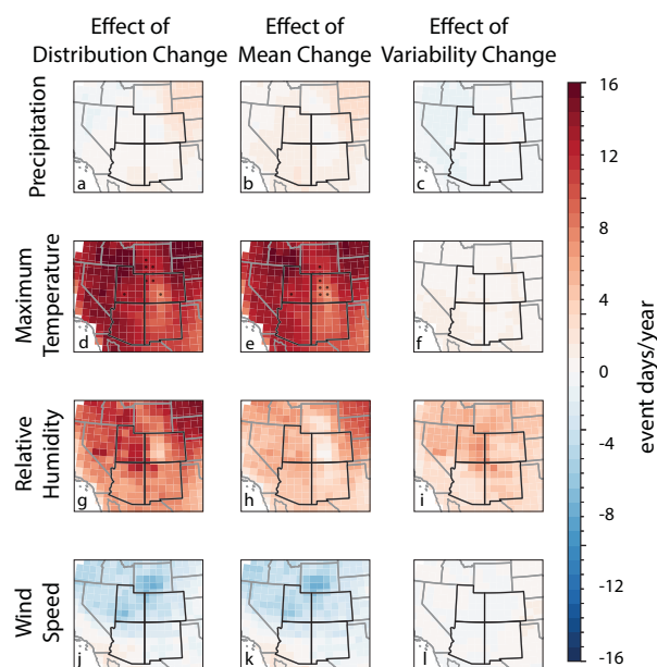
FIG. 11. The effect of changes in the (a),(d),(g),(j) distribution, (b),(e),(h),(k) mean, and (c),(f),(i),(l) variability of (a)–(c) precipitation, (d)–(f) maximum temperature, (g)–(i) relative humidity, and (j)–(l) wind speed on changes (from the historic period, 1980–2014) in the number of event days per for the Four Corners region for JJASO in the late future period (2050–82) (see supplemental Fig. 2 for details of the effect calculation for each FWI variable). These composites are created by averaging event characteristics for all events for each ensemble member for each period at each grid point. Then, the gridpoint-specific values of the historic period are subtracted from the late future period for each ensemble member, and the difference values are averaged over all ensemble members. Stippling indicates that the difference from the historic impacts is not significantly different ( p < 0.05 ). Results for event frequency, area, and intensity can be found in supplemental Fig. 7.
