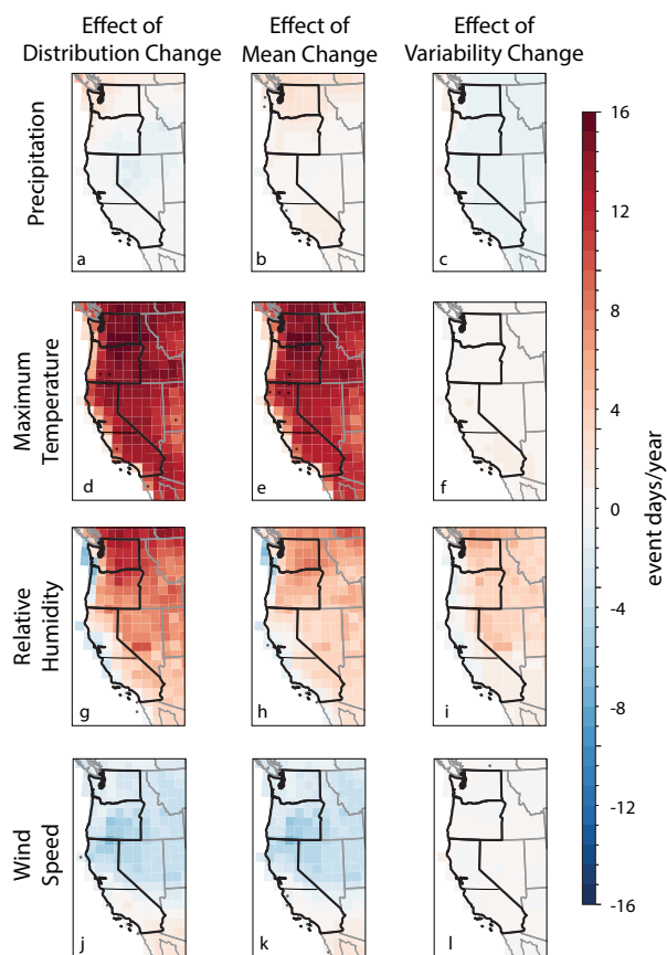
FIG. 9. The effect of changes in the (a),(d),(g),(j) distribution, (b),(e),(h),(k) mean, and (c),(f),(i),(l) variability of (a)–(c) precipitation, (d)–(f) maximum temperature, (g)–(i) relative humidity, and (j)–(l) wind speed on changes (from the historic period, 1980–2014) in the number of event days per year for the Pacific Coast region for JJASO in the late future period (2050–82) (see supplemental Fig. 2 for details of the effect calculation for each FWI variable). These composites are created by averaging event characteristics for all events for each ensemble member for each period at each grid point. Then, the gridpoint-specific values of the historic period are subtracted from the late future period for each ensemble member, and the difference values are averaged over all ensemble members. Stippling indicates that the difference from the historic impacts is not significantly different ( p < 0.05 ). Results for event frequency, area, and intensity can be found in supplemental Fig. 6.
