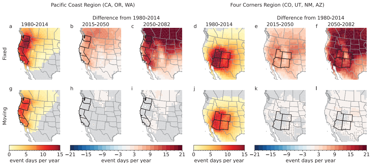
FIG. 3. Total number of event days per year over each grid point in the (a),(d),(g),(j) historic period (1980–2014) and change in the number of event days per year over each grid point in (b),(c),(e),(f),(h),(i),(k),(l) future periods using (a)–(f) fixed and (g)–(l) moving threshold for events fully or partially located in the (a)–(c),(g)–(i) Pacific Coast and in the (d)–(f),(j)–(l) Four Corners regions in JJASO. For the historic period, all shaded locations have at least 0.66 event days per year, meaning that at least two-thirds of the ensembles show 1 event day per year on average. Similarly, for the future period changes, all shaded locations have an increase or decrease of at least 0.33 event days per year. Stippling indicates that the difference from the historic period is not statistically significant ( p value \leq 0.05 ).
