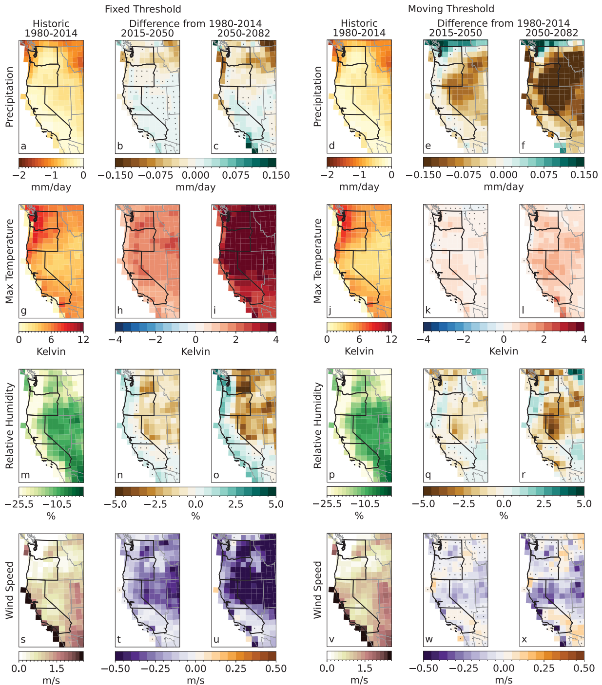
FIG. 5. (a),(d),(g),(j),(m),(p),(s),(v) Composite maps of precipitation ( \text{mm day}^{-1} ), maximum temperature (K), relative humidity (%), and wind speed ( \text{m s}^{-1} ) anomalies during extreme fire weather events using (a),(g),(m),(s) 30-day, 35-yr fixed mean for the fixed threshold events and (d),(j),(p),(v) 30-day, 35-yr moving mean for the moving threshold events in the Pacific Coast region in JJASO for the historic period (1980–2014). (b),(c),(e),(f),(h),(i),(k),(l),(n),(o),(q),(r),(t),(u),(w),(x) Composite maps showing the changes in these fire weather variables in the two future periods for the fixed and moving thresholds for 2015–50 and 2050–82. The composites are created by averaging the variable anomalies over the area and duration of all events across all ensemble members in each period. Stippling indicates that the difference from the historic period is not statistically significant ( p \text{ value} \leq 0.05 ).
