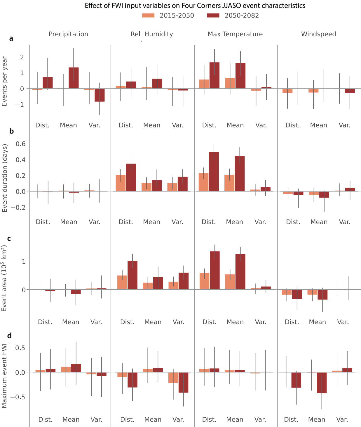
FIG. 12. The difference (from the historic period, 1980–2014) in the impact of changes in the full distribution (Dist.), mean, and variability (Var.) of precipitation, relative humidity, maximum temperature, and wind speed on (a) events per year, (b) events days per year, (c) regional event area, and (d) maximum regional event intensity FWI using the fixed threshold for the early (2015–50, coral) and late future periods (2050–82, red) for the Four Corners region in JJASO (see supplemental Fig. 2 for details of the effect calculation for each FWI variable). The mean across all events for each ensemble member is first calculated, and we show the median across all ensemble members. The error bar represents 25th–75th percentile of the ensemble spread.
