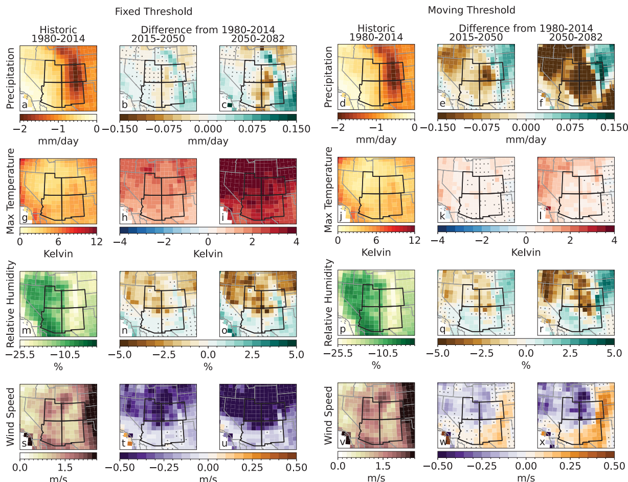
FIG. 7. (a),(d),(g),(j),(m),(p),(s),(v) Composite maps of precipitation ( \text{mm day}^{-1} ), maximum temperature (K), relative humidity (%), and wind speed ( \text{m s}^{-1} ) anomalies during extreme fire weather events using (a),(g),(m),(s) 30-day, 35-yr fixed mean for the fixed threshold events and (d),(j),(p),(v) 30-day, 35-yr moving mean for the moving threshold events in the Four Corners region in JJASO for the historic period (1980–2014). (b),(c),(e),(f),(h),(i),(k),(l),(n),(o),(q),(r),(t),(u),(w),(x) Composite maps showing the changes in these fire weather variables in the two future periods for the fixed and moving thresholds for 2015–50 and 2050–82. The composites are created by averaging the variable anomalies over the area and duration of all events across all ensemble members in each period. Stippling indicates that the difference from the historic period is not statistically significant ( p value \leq 0.05 ).
