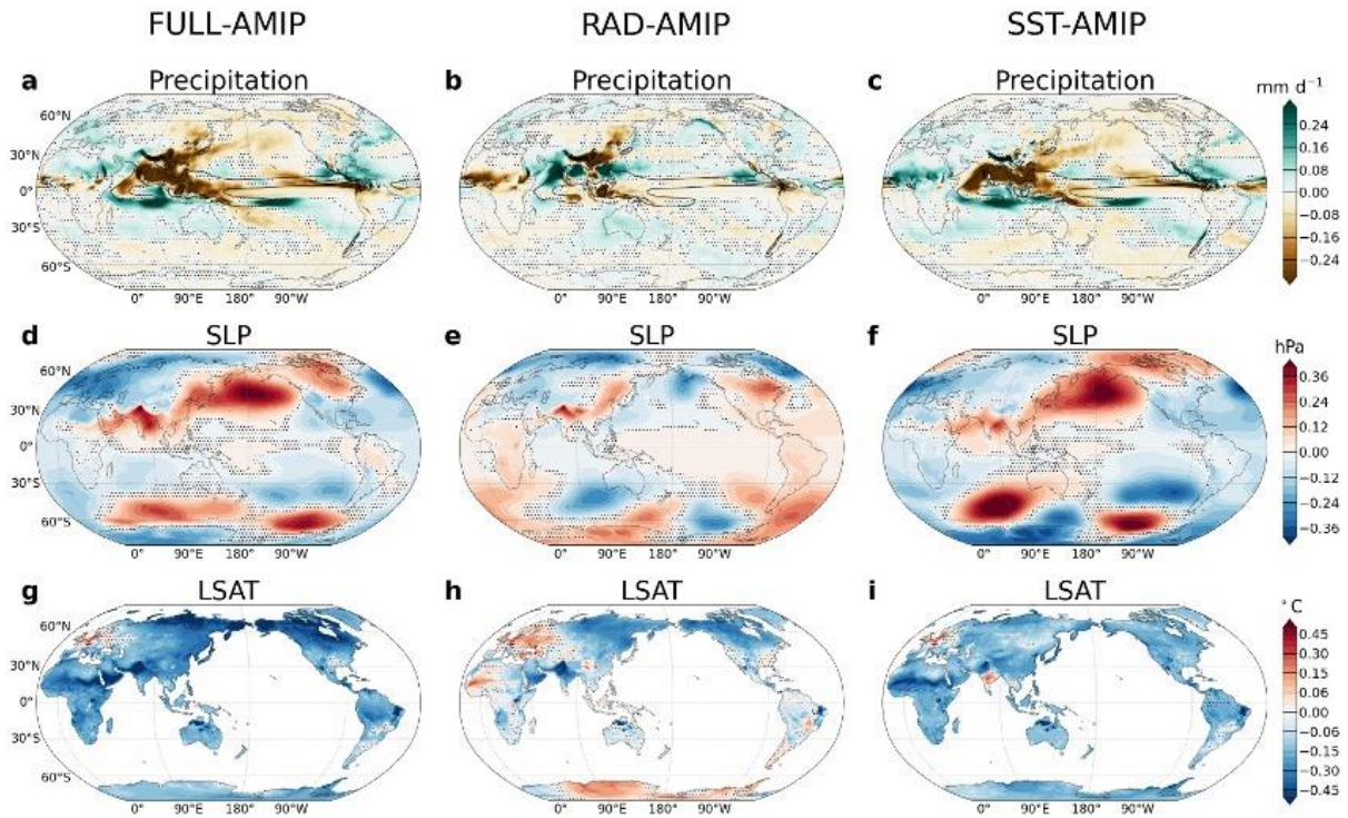
32 Figure S2. Regressions onto FULL-AMIP SST PC1: (a,b,c) precipitation (mm d -1 ), (d,e,f) sea level pressure 33 (SLP; hPa) and (g,h,i) land surface air temperature (LSAT; °C) in FULL-AMIP, RAD-AMIP and SST-AMIP. 34 Statistical significance of all regression values is assessed using a two-tailed Student's t-test with effective 35 degrees of freedom computed according to Bretherton et al. (1999) and applying the False Discovery Rate 36 (FDR) with control level \alpha_{FDR} = 0.05 to measure the field significance of the response (Wilks 2016).
