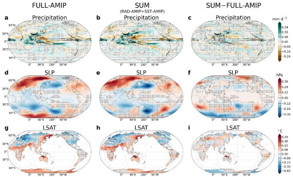
60 Figure S6. Additivity analysis based on AOD Mode 2. (a,d,g) FULL-AMIP, (b,e,h) the sum of RAD-AMIP 61 and SST-AMIP (SUM), and (c,f,i) the difference of SUM and FULL-AMIP. Statistical significance of all 62 regression values is assessed using a two-tailed Student's t -test with effective degrees of freedom computed 63 according to Bretherton et al. (1999) and applying the False Discovery Rate (FDR) with control level \alpha_{FDR} 64 = 0.05 to measure the field significance of the response (Wilks 2016). Black contours on precipitation panels 65 show the climatological 6 mm d -1 isopleth.
