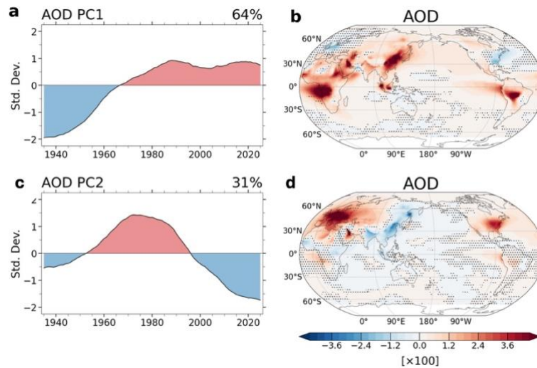
22 Figure S1. (a,c) Principal Component (PC) time series of 10-year low-pass filtered Aerosol Optical Depth 23 (AOD) in JJA based on RAD-AMIP. Percent variance explained by Modes 1 and 2 (PC1 and PC2) are given 24 in the upper right. (b,d) Regression of JJA AOD ( \times 100 ) in RAD-AMIP onto AOD PC1 and PC2. Statistical 25 significance of all regression values is assessed using a two-tailed Student's t-test with effective degrees of 26 freedom computed according to Bretherton et al. (1999) and applying the False Discovery Rate (FDR) with 27 control level \alpha_{FDR} = 0.05 to measure the field significance of the response (Wilks 2016).
