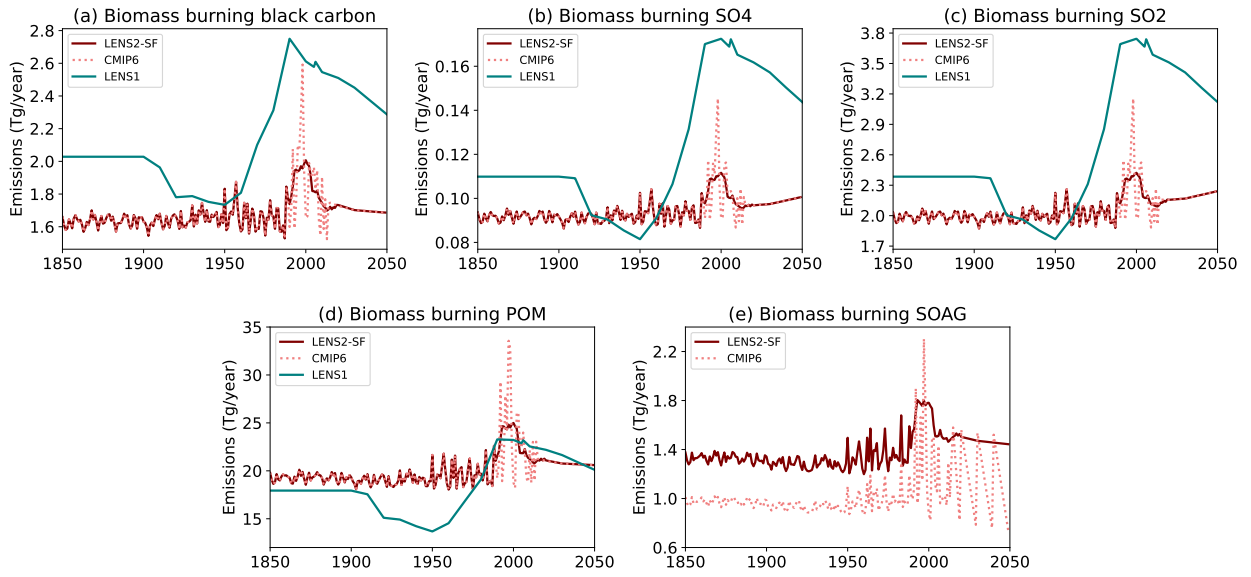
14 FIG. 1. A comparison of biomass burning emissions of (a) black carbon, (b) SO 4 , (c) SO 2 , (d) Primary Organic Matter (POM), 15 and (e) Secondary Organic Aerosol precursor Gases (SOAG) between LENS1 (teal), the CESM2 single forcing large ensemble 16 (maroon solid) and the CMIP6 historical and SSP3-7.0 biomass burning emissions (dotted salmon). Note that LENS1 is not shown 17 for SOAG as it was not possible to divide SOAG emissions up into the different components in the same way in CESM1. Note 18 also that for SOAG, the differences in emissions between CMIP6 and the single forcing large ensemble reflects a correction to the 19 CESM2 SOAG emissions between the first and second 50 members of LENS2 (Rodgers et al. 2021).
