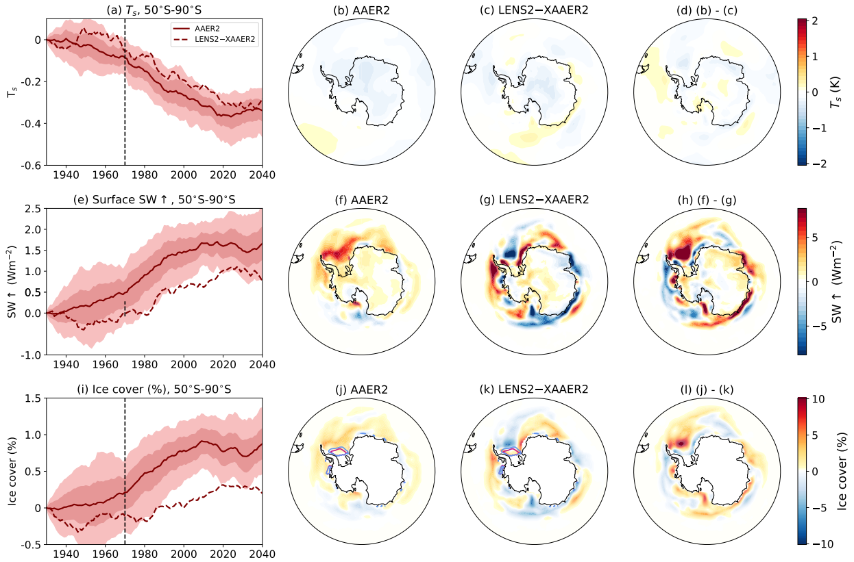
36 FIG. 8. (a)-(d) show DJF averaged near surface air temperature. (a) shows time series of 50^{\circ}S - 90^{\circ}S average anomalies from 37 1920-1940. (b) Shows the anomalies for 1960-1980 for AAER2, (c) shows the anomalies for 1960-1980 for LENS2-XAAER2 38 and (d) shows the difference in anomalies between AAER2 and LENS2-XAAER2. (e)-(h) are as (a)-(d) but for surface upward 39 shortwave radiation and (i)-(l) are as (a)-(d) but for the average percentage cover of sea ice in each grid point. The blue and purple 40 contours in (j) and (k) show the 80% ice coverage contours for 1920 to 1940 of AAER2 and 1960 to 1980 of XAAER2 respectively.
