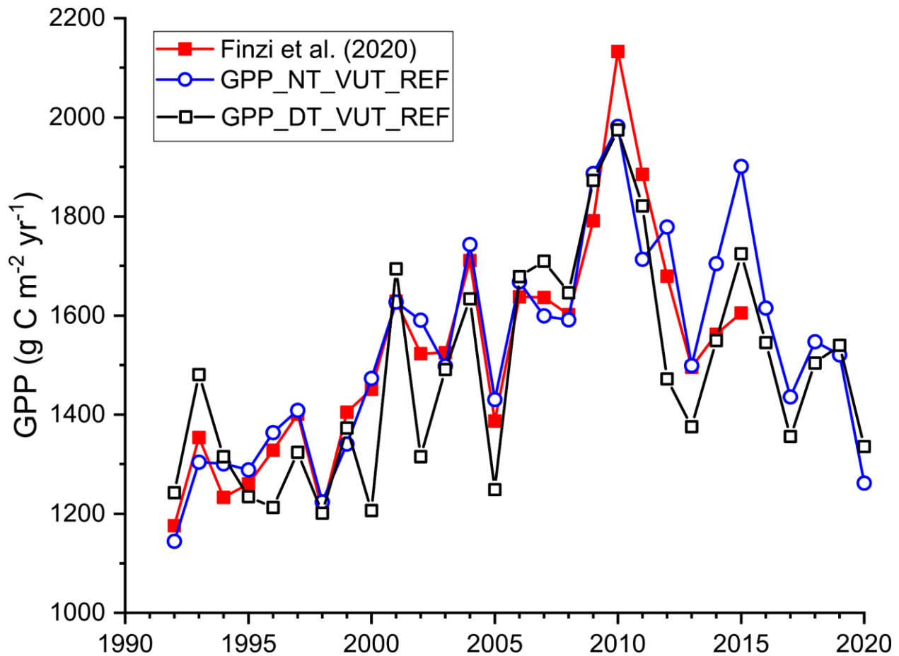
165 Supplementary Fig. 10. Estimates of annual gross primary production (GPP) at the AmeriFlux US-Ha1 166 (Harvard Forest) flux tower. Data are from Finzi et al. (2020) (ref. 19) for 1992–2015 and the AmeriFlux 167 (Munger, 2022) database (ref. 52) for 1992–2020 using the GPP_NT_VUT_REF and GPP_DT_VUT_REF 168 products. The two products differ in nighttime (NT) and daytime (DT) partitioning of net ecosystem 169 exchange to obtain GPP. The GPP_NT_VUT_REF product compares favorably with the Finzi et al. data.
