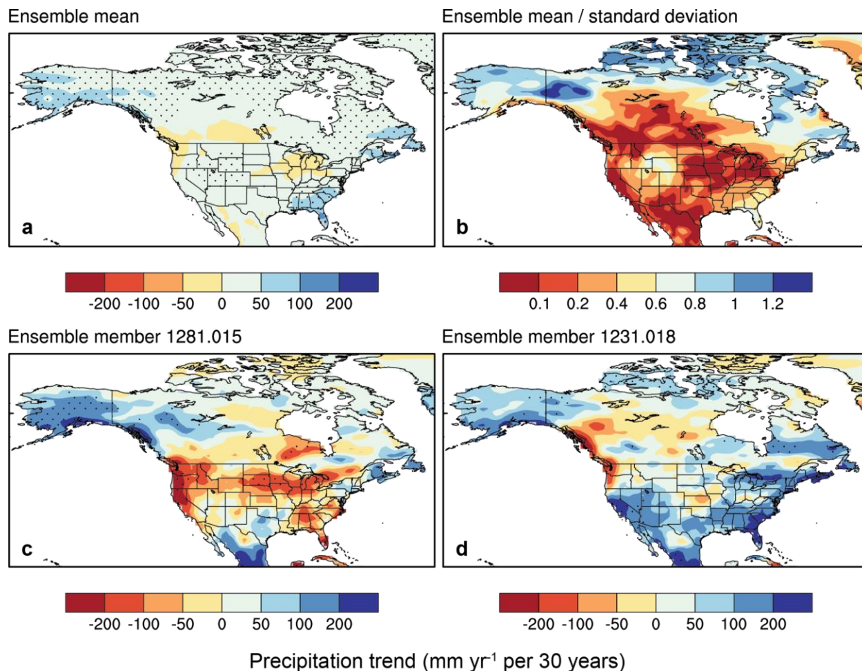
124 Supplementary Fig. 8. Trends in annual precipitation for 1991–2020. (a) Mean trend for the 50- 125 member ensemble obtained from the ensemble mean time series. (b) Signal-to-noise ratio defined as 126 the ensemble mean trend (absolute value) divided by the standard deviation of trends across the 50 127 members. Also shown are trends for two members with small (c) and large (d) continental mean trends. 128 Ensemble members 1281.015 and 1231.018 are the members at the 3rd (6th percentile) and the 47th 129 (94th percentile) ranks, respectively, based on continental mean trends. Stippling denotes statistical 130 significance ( n = 30 years; p \leq 0.05 ) using the ensemble mean time series or the individual ensemble 131 member time series. Trends are multiplied by 30 to report the change in precipitation over the 30-year 132 period.
