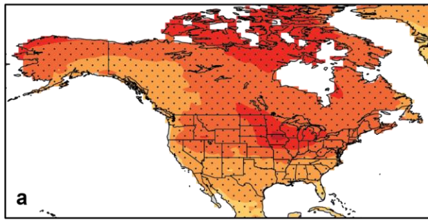
Ensemble mean
