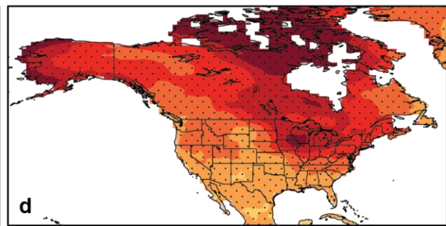
Ensemble member 1011.001
