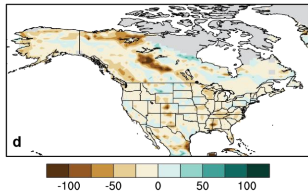
Ensemble member 1231.018
