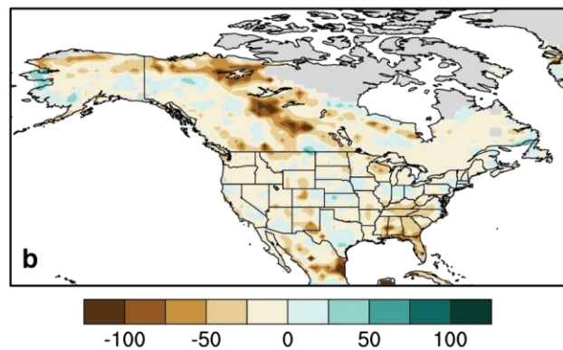
Ensemble member 1251.011
