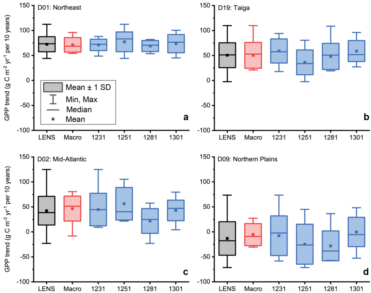
142 Supplementary Fig. 9. Box plots of annual GPP trends for 1991–2020. Trends are given for the full 50- 143 member large ensemble (LENS), the 10-member macro-initialization (Macro), and the four micro- 144 initializations with 10-members each (start years 1231, 1251, 1281, and 1301 of the preindustrial 145 control). Plotted are the mean ± one standard deviation, the minimum and maximum, the median, and 146 the mean. Trends are shown for the grid cells corresponding to NEON core terrestrial sites for (a) D01: 147 Northeast, (b) D19: Taiga, (c) D02: Mid-Atlantic, and (d) D09: Northern Plains. These are the four grid 148 cells in Fig. 2.
