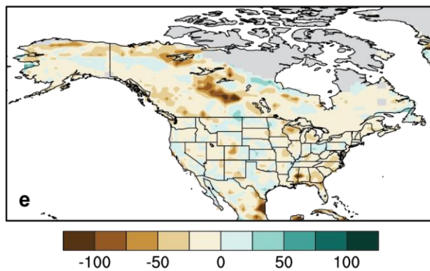
Ensemble member 1281.015
