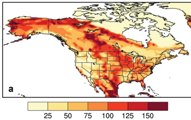
Ensemble member 1301.015
