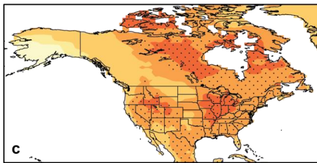
Ensemble member 1301.013
