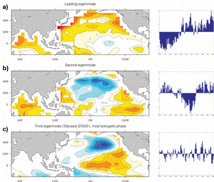
FIG. 4. (left) Leading empirical eigenmodes and (right) their corresponding time series from the LIM of annual-mean HadISST SST anomalies. The LIM is constructed as in Newman (2007), except that the EOF basis is determined over the entire Pacific domain (20°S–60°N); the leading 12 PCs are retained, explaining 92% of the variance in both the tropics and in the North Pacific, unlike in Newman (2007), where less than two-thirds of the North Pacific variance was retained. Contour interval is the same in all panels but is arbitrary. Red (blue) shading indicates positive (negative) values; zero contour is removed for clarity. (a) Leading eigenmode, stationary with decay time of 13 yr. (b) Second eigenmode, stationary with decay time of 6.4 yr. (c) Most energetic phase of third (“decadal ENSO”) eigenmode, propagating with a period of 16 yr and decay time of 2.1 yr.
