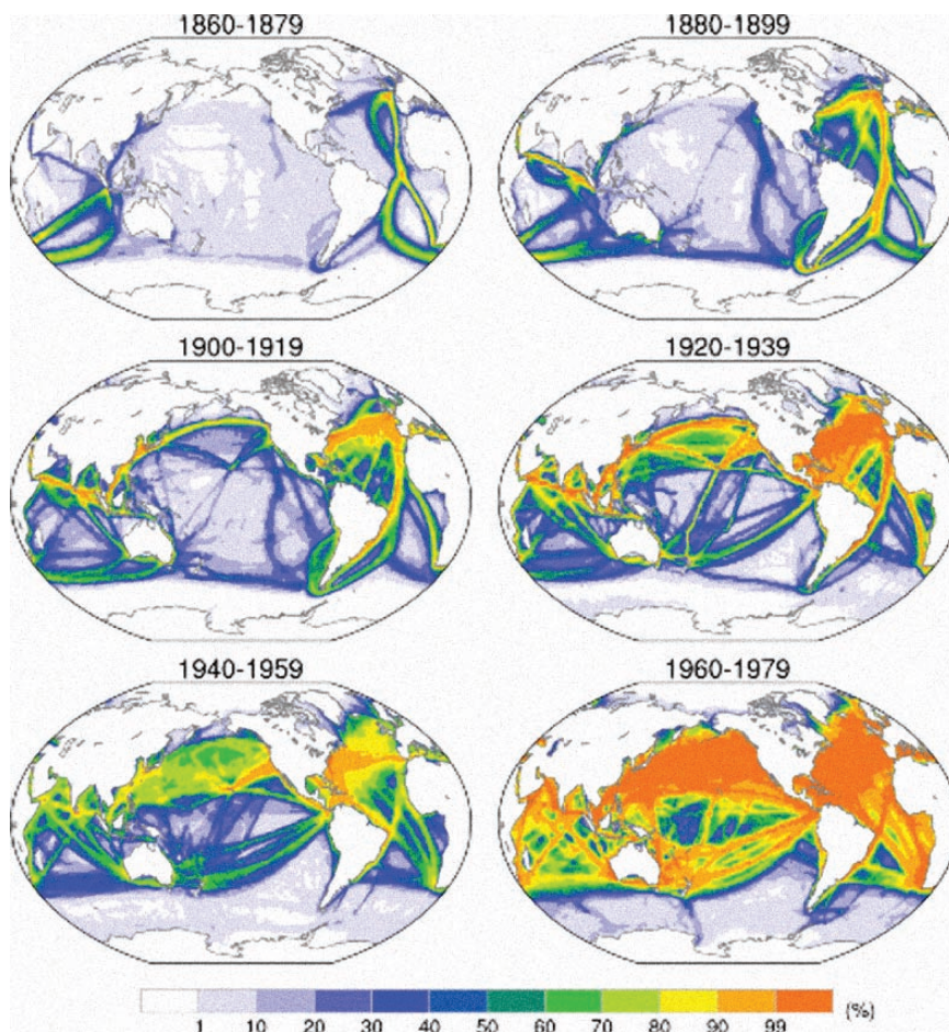
FIG. 6. Distribution of surface marine observations from the International Comprehensive Ocean-Atmosphere Data Set (ICOADS), shown as the percent of months with at least one observation per 2^{\circ} lat \times 2^{\circ} lon grid box during the 20-yr period indicated. Adapted from Deser et al. (2010a).
