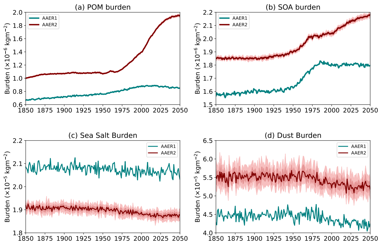
FIG. 4. Globally averaged aerosol burden in the AAER1 (teal) and AAER2 (maroon) experiments. The uncertainty range estimated by bootstrapping the AAER2 ensemble members with replacement is shown for the 15 member AAER2 ensemble in the dark shading and for a 3 member ensemble in light shading.
