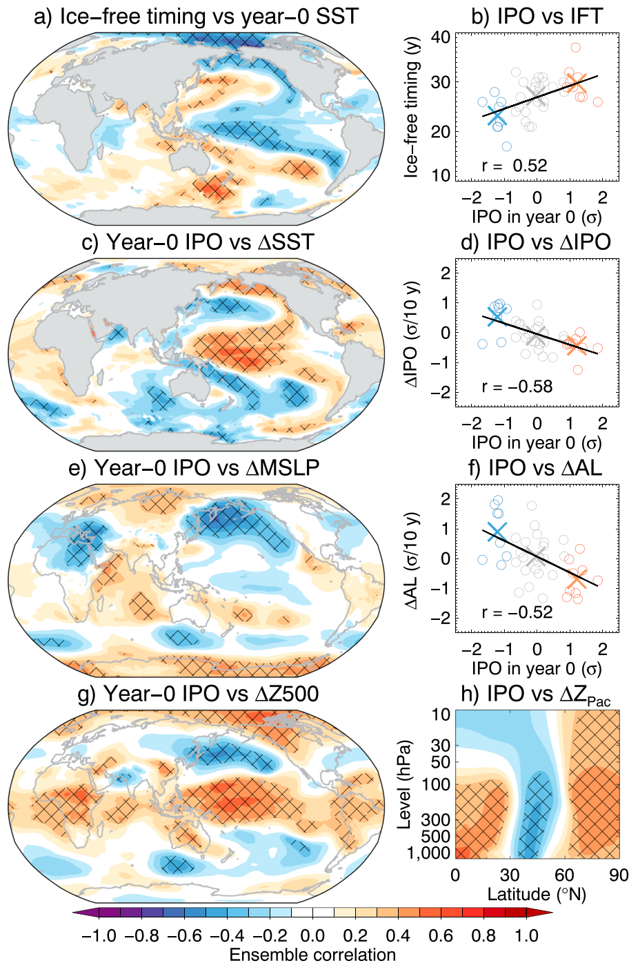
Figure 2. Internal climate variability linked to faster sea-ice loss. (a) Ensemble correlation between the time of emergence of an ice-free Arctic and annual-mean sea surface temperatures (SST) in year 0 of each trajectory. Black hatching shows statistical significance at the 95% confidence level ( p < 0.05 ). The sign of the correlations has been reversed to display the pattern linked to an earlier emergence of ice-free conditions. (b) Relationship between the timing of ice-free conditions and the Interdecadal Pacific Oscillation (IPO) index in year 0. There are 40 circles, one per trajectory, which are colored according to the IPO index in year 0 (as in Figure 1). The black line denotes the linear best fit, and the colored crosses show averages for the three IPO categories Ice-free timing (IFT). (c) As (a), but for the ensemble correlation between the IPO index in year 0 and the annual-mean SST trend in each trajectory. (d) As (b), but for the relationship between the IPO index in year 0 and the IPO trend. (e) As (c), but for the correlation between the IPO index in year 0 and the cold season (October–March) mean sea level pressure (MSLP) trend. (f) As (d), but for the relationship between the IPO index in year 0 and the cold season Aleutian Low (AL) trend. (g) As (c), but for the relationship between the IPO index in year 0 and the 500-hPa geopotential height (Z500) trend. (h) Ensemble correlation between the IPO index in year 0 and the geopotential height trend zonally averaged over the Pacific sector ( Z_{\text{Pac}} ). In (a, c, f, g), the sign of the correlations has been reversed to display the patterns linked to negative IPO in year 0.
