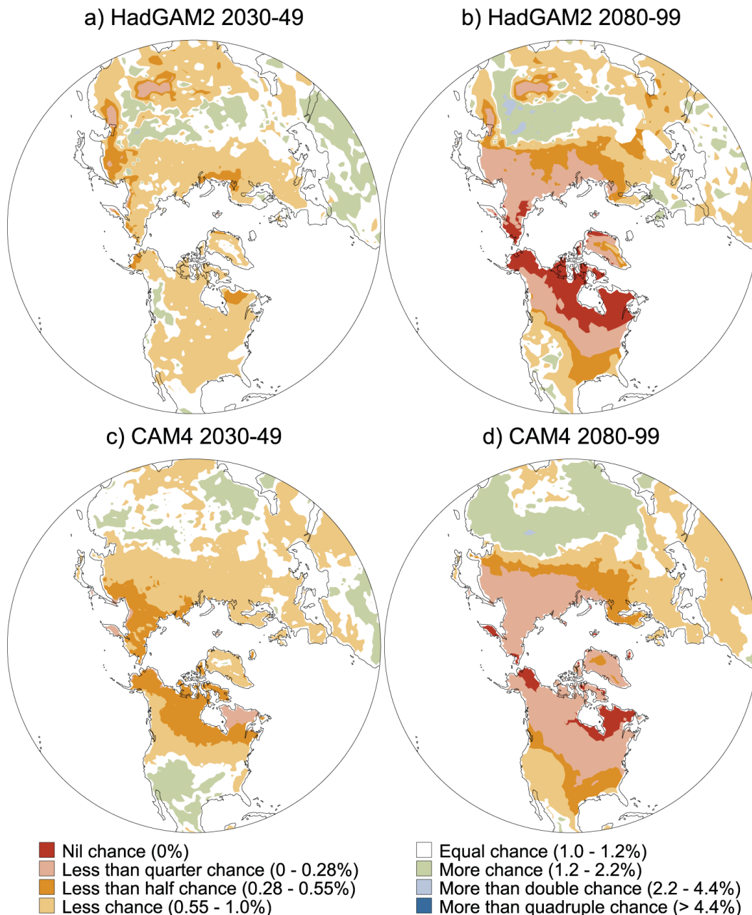
FIG. 7. (a) Probability of extreme cold (winter daily temperature as cold or colder than the 1.1 percentile during the period 1980–99) in the sea ice–forced HadGAM2 simulation for the period 2030–49. Colored shading categories are based on the relative change in probability compared to the period 1980–99. (b) As in (a), but for the period 2080–99 relative to 1980–99. (c),(d) As in (a),(b), but for the sea ice–forced CAM4 simulations.
