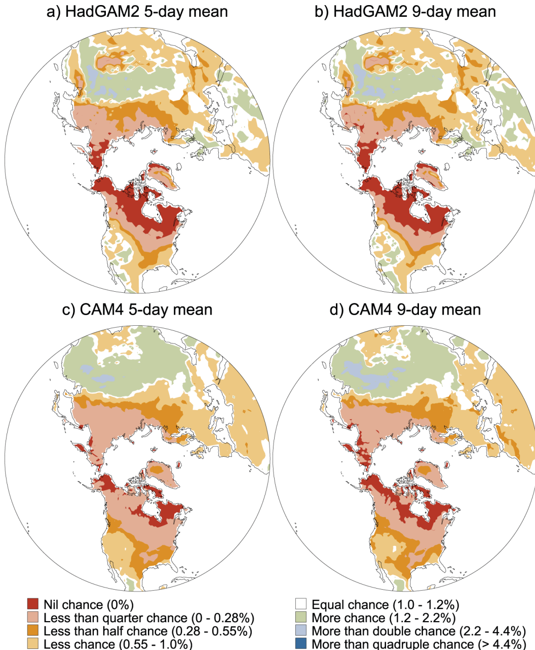
FIG. 8. (a) Probability of extreme cold (winter 5-day mean temperature as cold or colder than the 1.1 percentile during the period 1980–99) in the sea ice–forced HadGAM2 simulation for the period 2080–99. Colored shading categories are based on the relative change in probability compared to the period 1980–99. (b) As in (a), but for 9-day means. (c),(d) As in (a),(b), but for the sea ice–forced CAM4 simulations.
