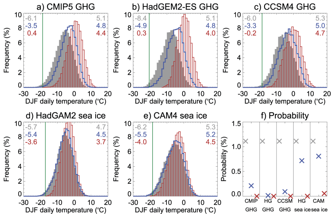
FIG. 4. (a) Histograms of simulated daily winter temperature averaged over CENA taken from 34 coupled climate models for the periods 1980–99 (gray bars), 2030–49 (blue), and 2088–99 (red). Numbers in the top left and top right of each panel are the mean temperature (°C) and standard deviation (°C), respectively. Vertical green line denotes the value of the model's 1.1 percentile, the simulated analog of the 7 Jan 2014 event in observations. (b)–(e) As in (a), but for coupled simulations with (b) HadGEM2-ES and (c) CCSM4 and for sea ice–forced simulations with (d) HadGAM2 and (e) CAM4. (f) Probability of daily temperature as cold or colder than the 1.1 percentile in the period 1980–99 in each model ensemble and period.
