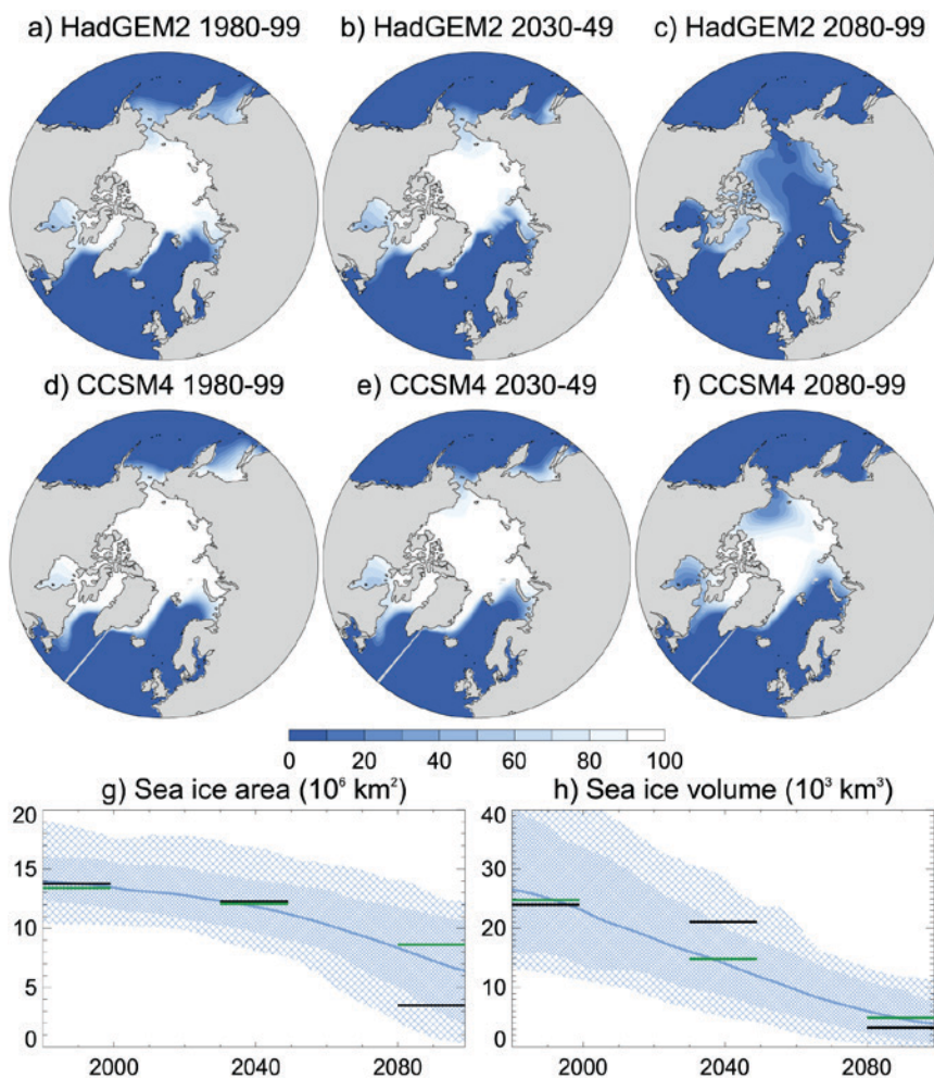
FIG. 3. Ensemble-mean winter sea ice concentrations from HadGEM2-ES during the period (a) 1980–99, (b) 2030–49, and (c) 2080–99. (d)–(f) As in (a)–(c), but for CCSM4. (g) Evolution of winter sea ice area in the CMIP5 historical and RCP8.5 experiments, 1980–2099. Blue curve denotes the multimodel mean, dense hatching denotes the 10%–90% range of the model spread, and light hatching denotes the full model spread. Black and green lines show the values prescribed in the sea ice–forced HadGAM2 and CAM4 simulations, respectively. (h) As in (g), but for sea ice volume.
