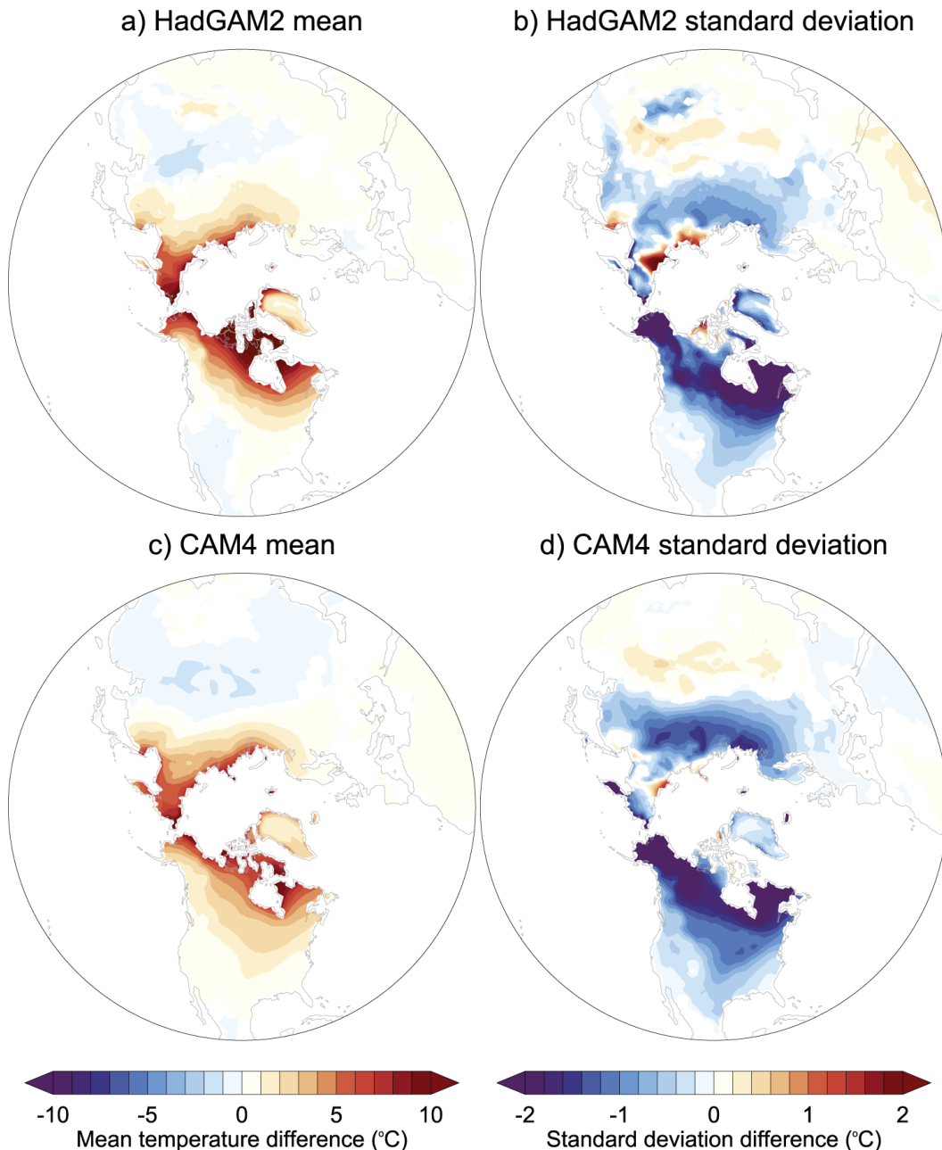
FIG. 6. As in Fig. 5, but for differences between the period 2080–99 and 1980–99. Note the different color scales.
