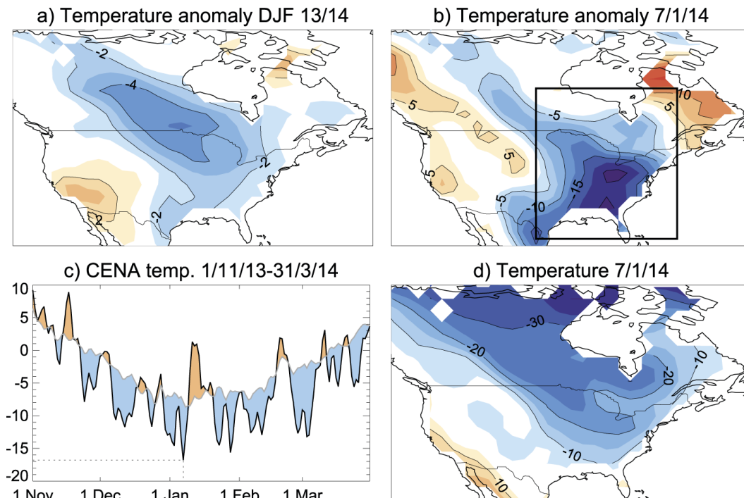
FIG. 1. North American temperature anomalies for (a) the winter of 2013/14 and (b) 7 Jan 2014. Anomalies are relative to the period 1980–99. (c) Daily mean temperature averaged over CENA [black box in (b)] for 1 Nov 2013–31 Mar 2014 (black curve) and the daily 1980–99 climatology (gray line). Blue (orange) shading shows days colder (warmer) than the average for that day. (d) North American temperatures for 7 Jan 2014.
