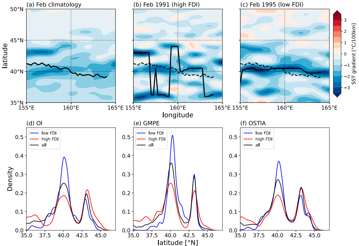
FIG. 6. February-mean poleward SST gradient (color shading; ^{\circ}\text{C} per 100 km) for (a) February climatology 1982–2016, (b) February 1991 (a high FDI case), and (c) February 1995 (a low FDI case) from the OI SST dataset. In (a), the locations of the maximum absolute SST gradients are shown with a black solid line which is drawn as black dashed lines in (b) and (c) extending only to 164^{\circ}\text{E} (the extent of the FDI). Data are not detrended in (a)–(c). (d)–(f) Kernel density estimates of the distribution for latitudes of the February maximum absolute SST gradients, at each longitude and for each February in 1982–2016 for (d) OI, (e) GMPE, and (f) OSTIA. Blue (red) curves show the third of months with the lowest (highest) FDI, and black curve is for all the February months.
