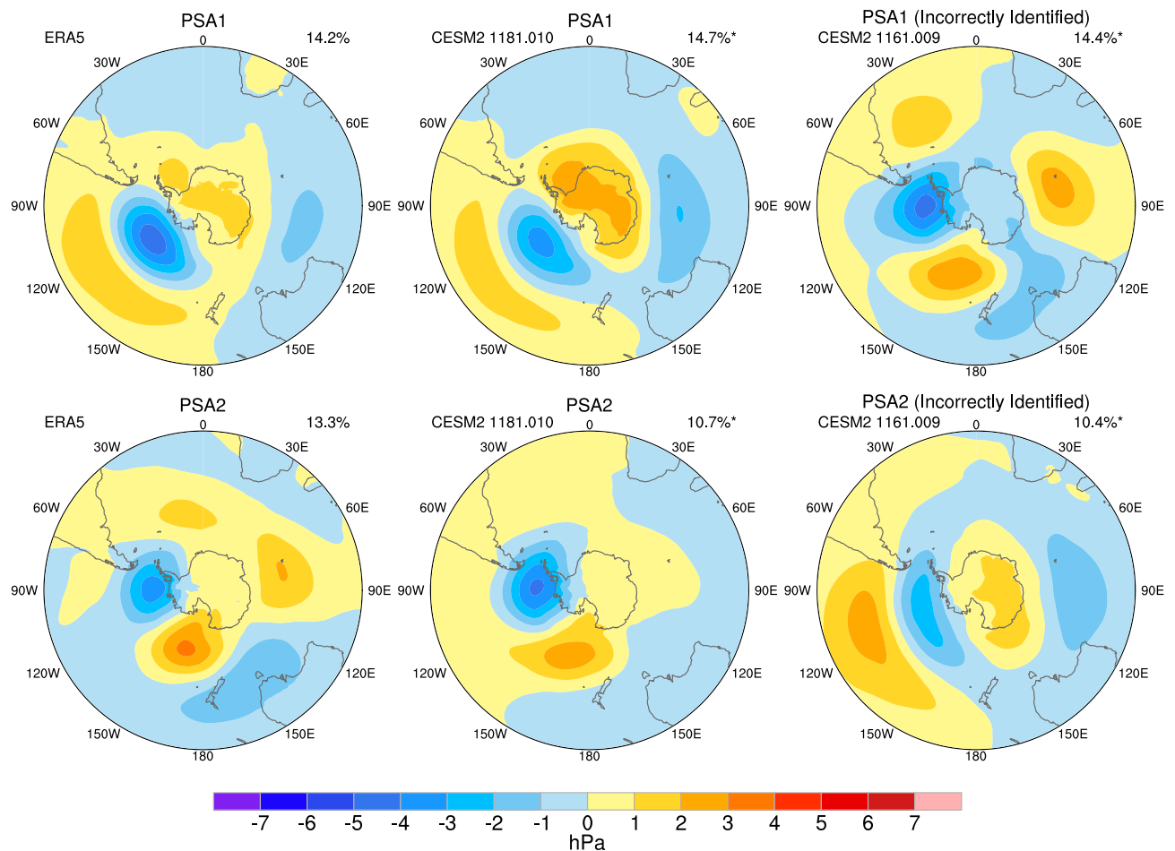
Fig. 2. Pacific South American (PSA) modes 1 (row 1) and 2 (row 2) shown for ERA5 (first column), CESM2 large ensemble member 1181.010 (second column) and CESM2 large ensemble member 1161.009 (third column). Mode swapping is evident in the third column. PSA1 and PSA2 are defined as the 2nd and 3rd EOF patterns of area-weighted PSL computed over 20°90°S, 0°360°E for June–August 1950–2023. Units are in hPa and variance explained is listed at the top right of each panel. The patterns are created by regressing global PSL anomalies onto normalized PC timeseries.
