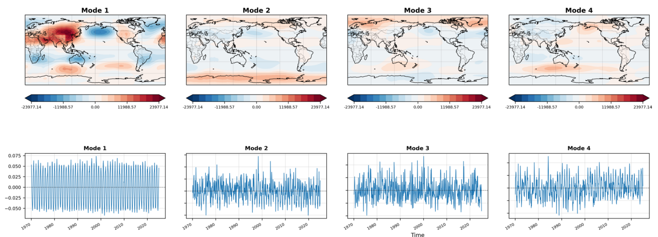
Fig. 11. As in Fig. 9, except using all core weights in combination.
