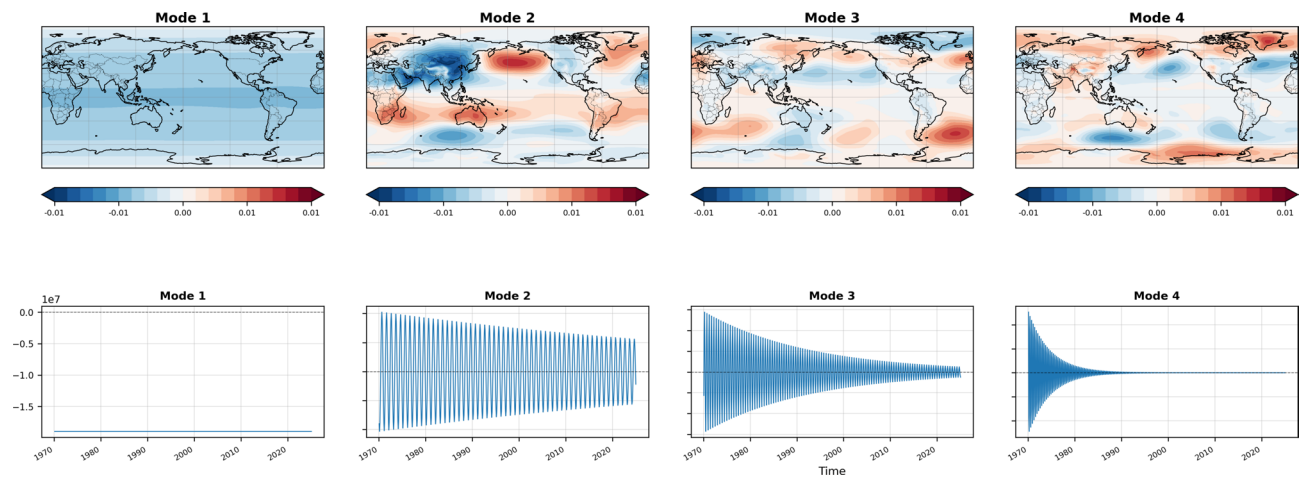
Fig. 19. As in Fig. 6, but for dynamic mode decomposition.
