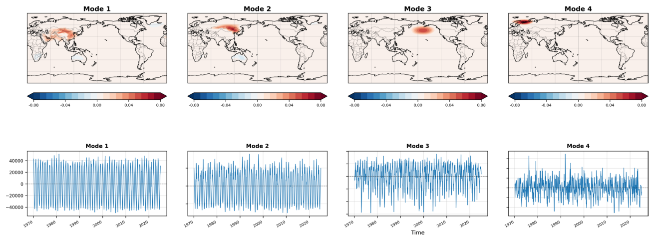
Fig. 15. As in Fig. 13, but an example of sparse EOF, where \alpha = 10,000 .
