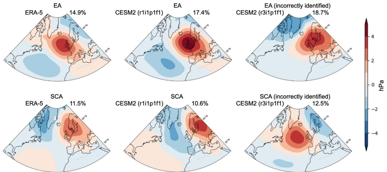
Fig. 1. East Atlantic pattern (EA, row 1) and Scandinavian pattern (SCA, row 2) shown for ERA5 (first column), CESM2 ScenarioMIP ensemble member r1i1p1f1 (second column) and CESM2 ScenarioMIP ensemble member r3i1p1f1 (third column). Mode swapping is evident in the third column. EA and SCA are defined as the 2nd and 3rd EOF patterns of area-weighted PSL computed over 20:80°N, -90:40°E for JFM 1979–2022. Units are in hPa and variance explained is listed at the top right of each panel.
