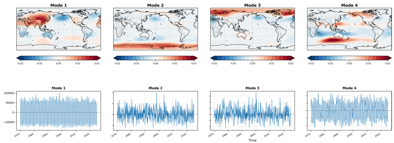
Fig. 13. As in Fig. 6, but an example of Sparse EOF, where \alpha = 1000 .
