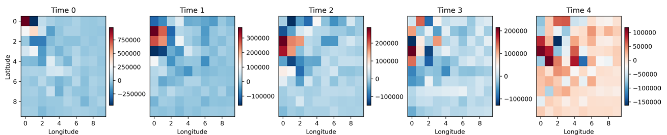
Fig. 9. Tucker decomposition core tensor of PSL CESM2 large ensemble member in Fig. 6, with a multirank of (5, 10, 10), with temporal modes 0 through 4, 10 latitudes (y-axis) and 10 longitudes (x-axis).
