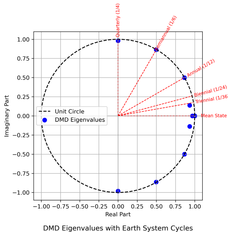
Fig. 18. Leading eigenvalue with earth system cycles (mean state, triennial, biennial, annual, semiannual, quarterly) sorted by magnitude. Blue circles represent DMD eigenvalues and the black dashed line is a unit circle for reference.
