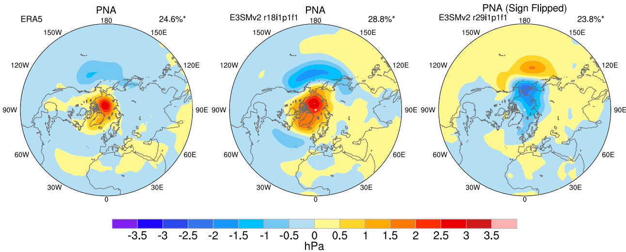
Fig. 3. Pacific North American pattern shown for ERA5 (first panel), E3SMv2 member r18i1p1f1 (second panel) and E3SMv2 member r29i1p1f1 (third panel). Sign flipping is evident in the third panel. Units are in hPa and variance explained for each pattern is listed at the top right. The PNA is defined as the first EOF pattern of area-weighted PSL computed over 20:85°N, 120°E:120°W for June–August 1950–2022. Units are in hPa and variance explained is listed at the top right of each panel. The patterns are created by regressing global PSL anomalies onto normalized PC timeseries.
