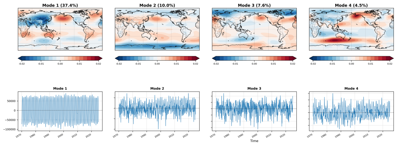
Fig. 6. PSL EOFs 1,2,3,4 (with percent variance explained) and respective PC timeseries for CESM2 model large ensemble, first member. No temporal filtering is done for consistency and comparison across alternative methods. See the "Methods" section under EOF: Standard Computation for an illustration on the potentially large differences due to temporal filtering.
