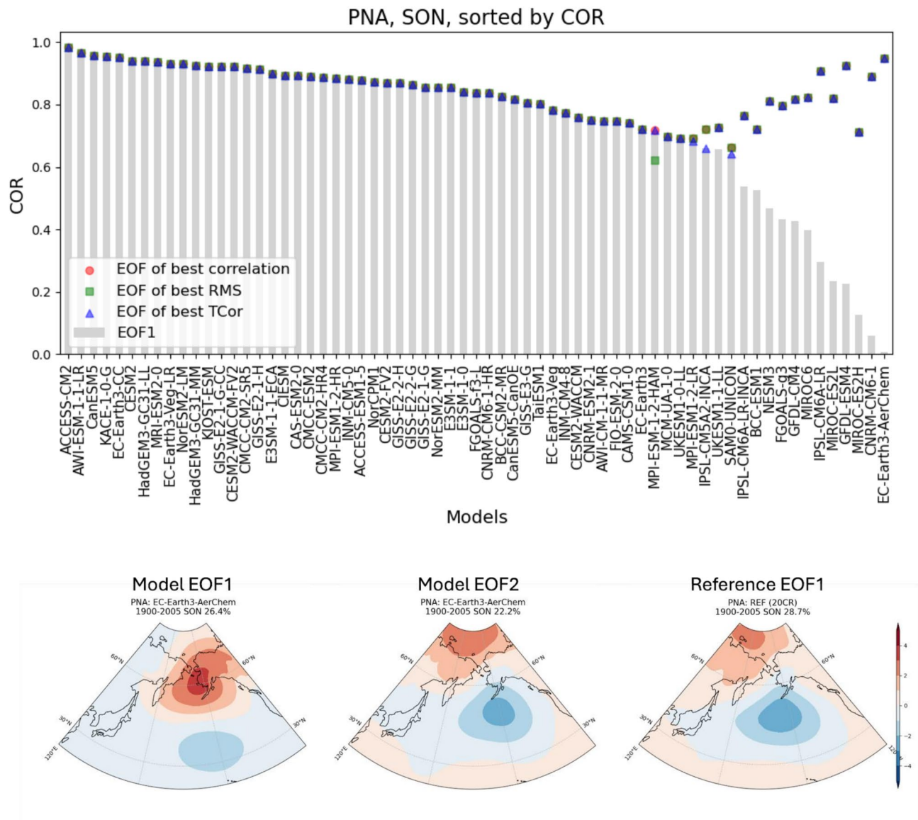
Fig. 5. Mode swapping pattern correlation adjustment method illustration. (Upper panel) Pattern correlation of CMIP6 models' Pacific/North American (PNA) pattern during the September–October–November (SON) season (upper panel). The PNA pattern for each model was determined by the leading empirical orthogonal function (EOF 1) of sea level pressure fields. Pattern correlation was then calculated between each model's EOF 1 spatial pattern and the 20th Century Reanalysis (20CR) PNA pattern (SON season). For each model, the pattern correlation of the leading three EOFs (EOF 1–3) was assessed against the 20CR PNA using spatial pattern correlation, Root Mean Square Error (RMSE), and temporal correlation between the EOF principal component (PC) time series and a Common Basis Function PC time series. The highest pattern correlation achieved after potentially swapping EOF modes based on these criteria is indicated by markers, while the pattern correlation of the original EOF 1 is shown as a gray bar. The increasing spread between EOF1 and the alternative EOF on the right demonstrates the difficulty in automated selection of the best-matching EOF mode for models on the right, which highlights challenges in systematically identifying robust climate patterns across different models (further details in Lee et al. 8 ). (Lower panel) Spatial pattern of model's EOF 1 (left), 2 (middle) and reference dataset's EOF 1 demonstrating an example EOF swap case, obtained from EC-Earth3-AerChem model (far-most right in the upper panel) and the 20CR for PNA pattern during the SON season. This figure is a modified and expanded version from Fig. 6 in Lee et al. 8 .
