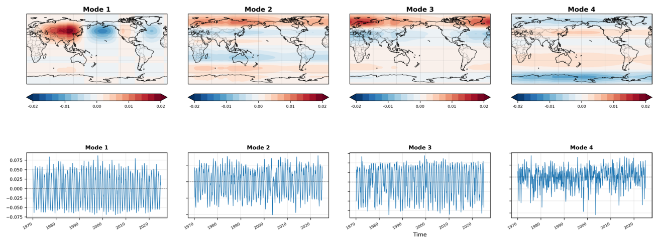
Fig. 20. As in Fig. 6, but for canonical polyadic decomposition using a low rank of R=4 .
