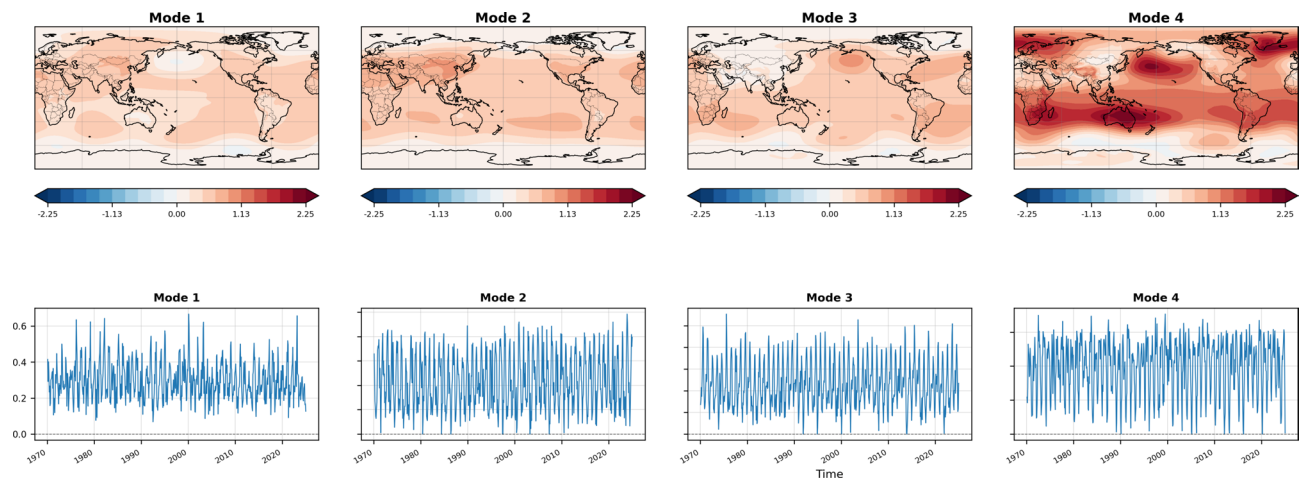
Fig. 17. As in Fig. 6, but for nonnegative matrix factorization.
