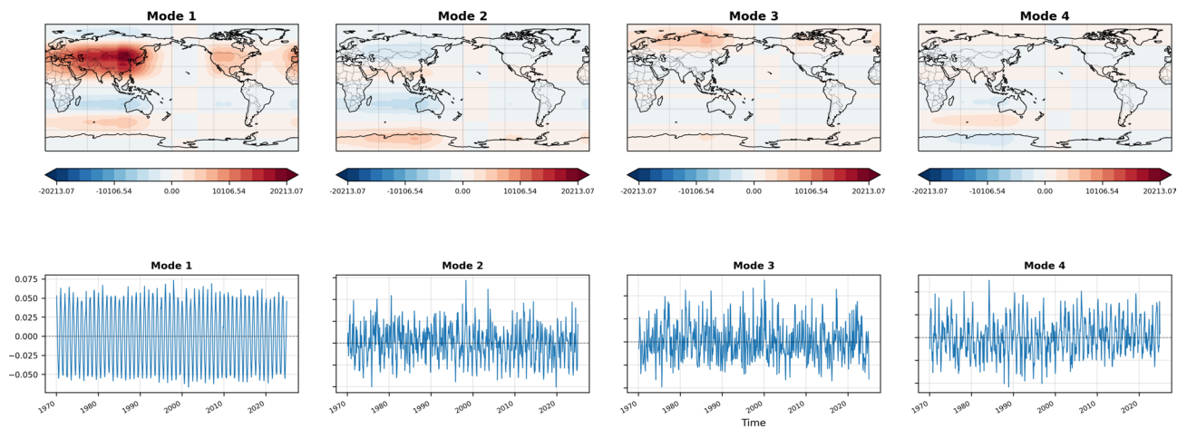
Fig. 10. As in Fig. 6, but for Tucker decomposition for the first four temporal components using the largest weights.
