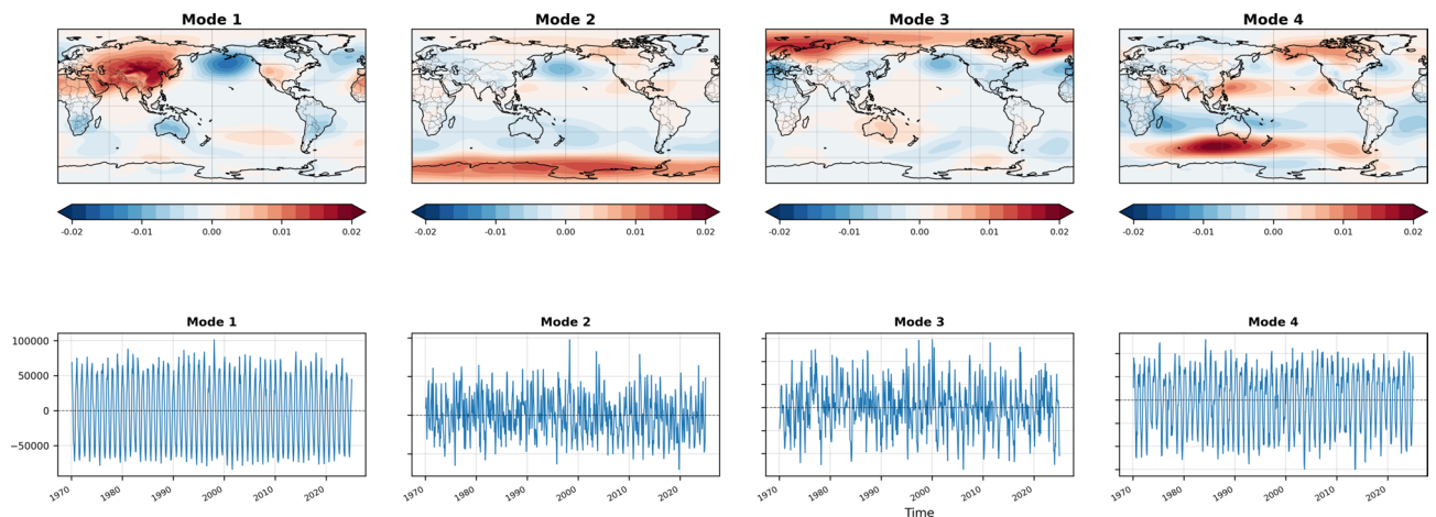
Fig. 7. As in Fig. 6, but an example of rotated EOF.
