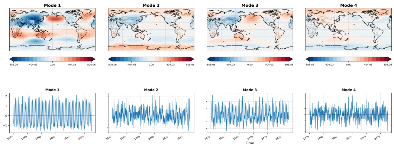
Fig. 8. As in Fig. 6 but using factor analysis.
