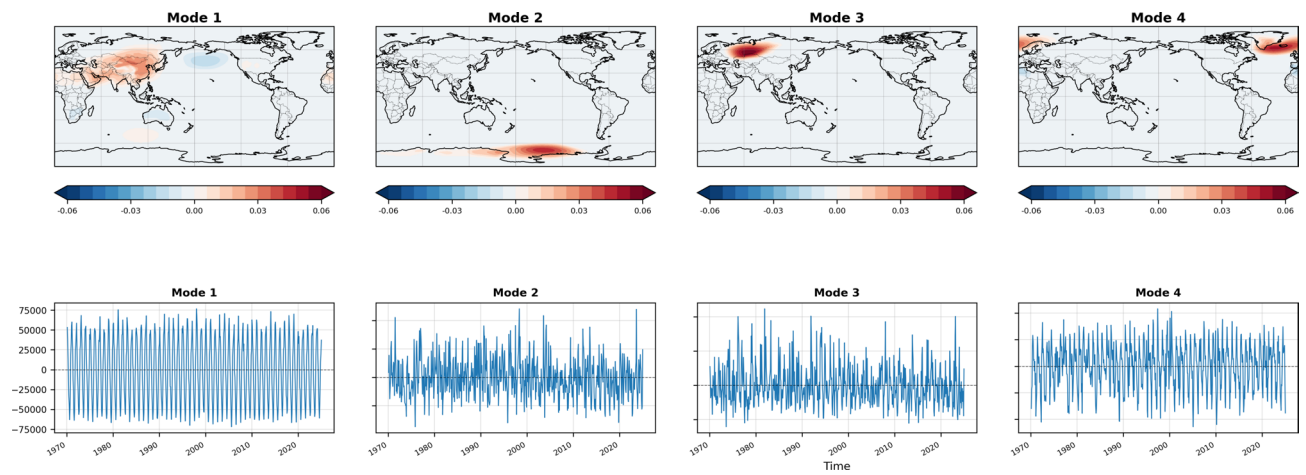
Fig. 14. As in Fig. 13, but an example of Sparse EOF, where \alpha = 7000 .
