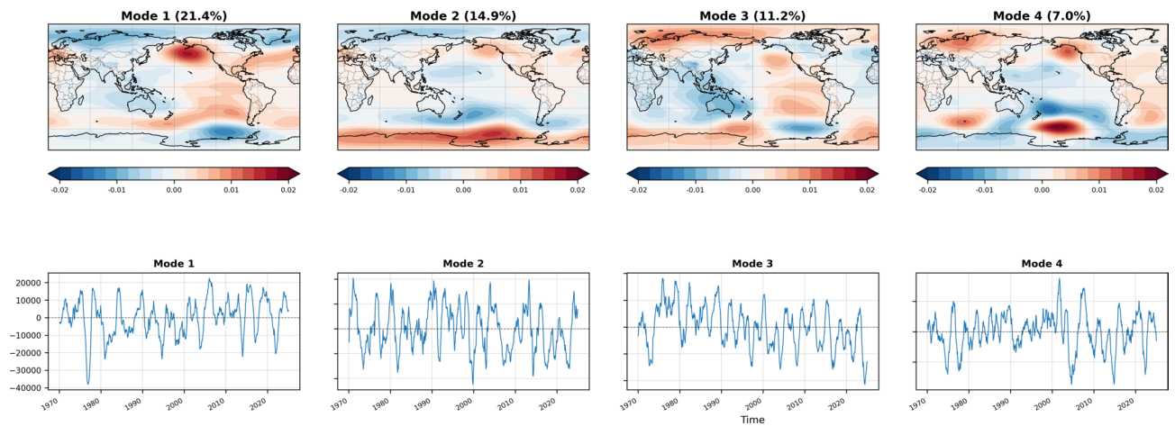
Fig. 12. As in Fig. 6, except using a 1-year rolling average to demonstrate the potentially large differences when temporal filtering is applied.
