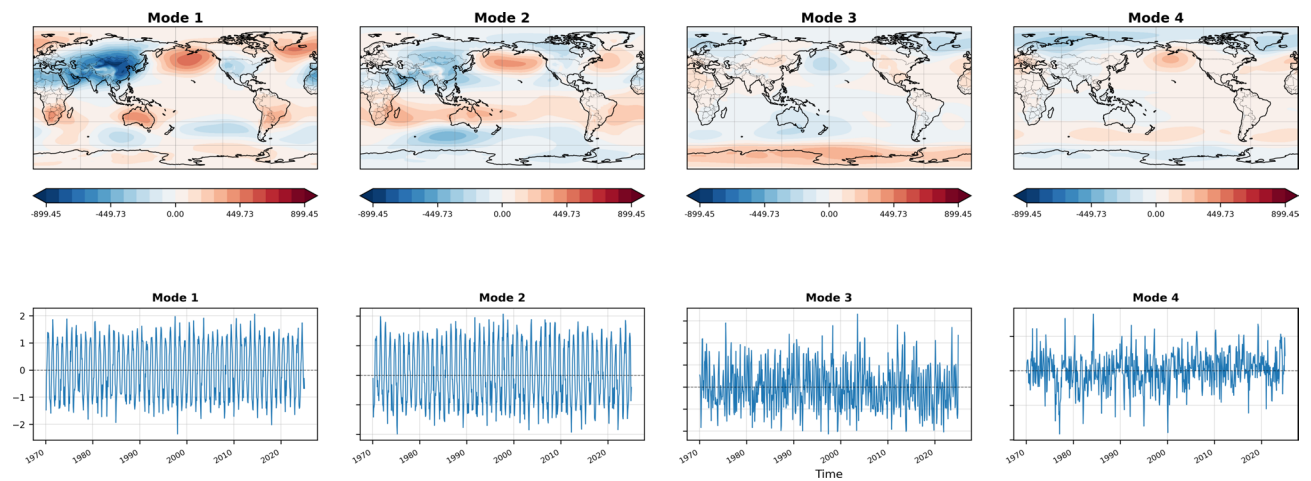
Fig. 16. As in Fig. 6, but for independent component analysis.
