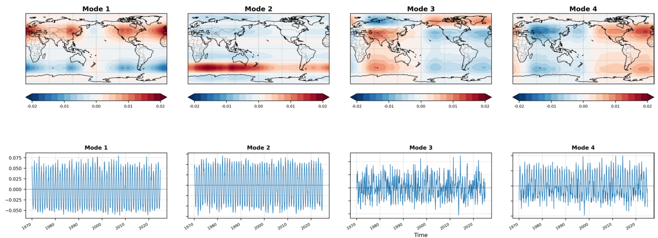
Fig. 21. As in Fig. 6, but for canonical polyadic decomposition using a high rank of R = 12 .
